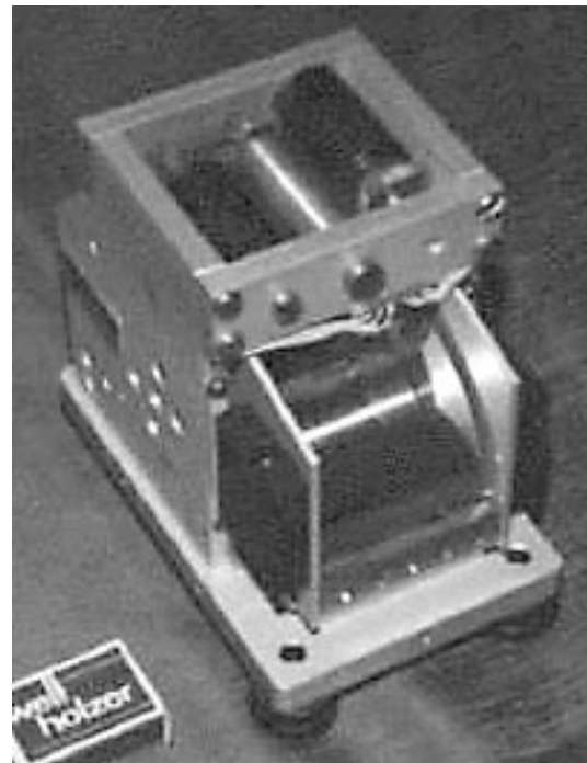
Fig. 2 Front view showing boom and seismic mass blocks
